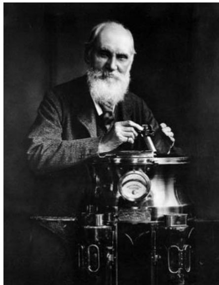
Lord Kelvin, 1883
